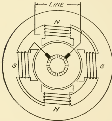
Fig. 29. Diagram of Series Motor
